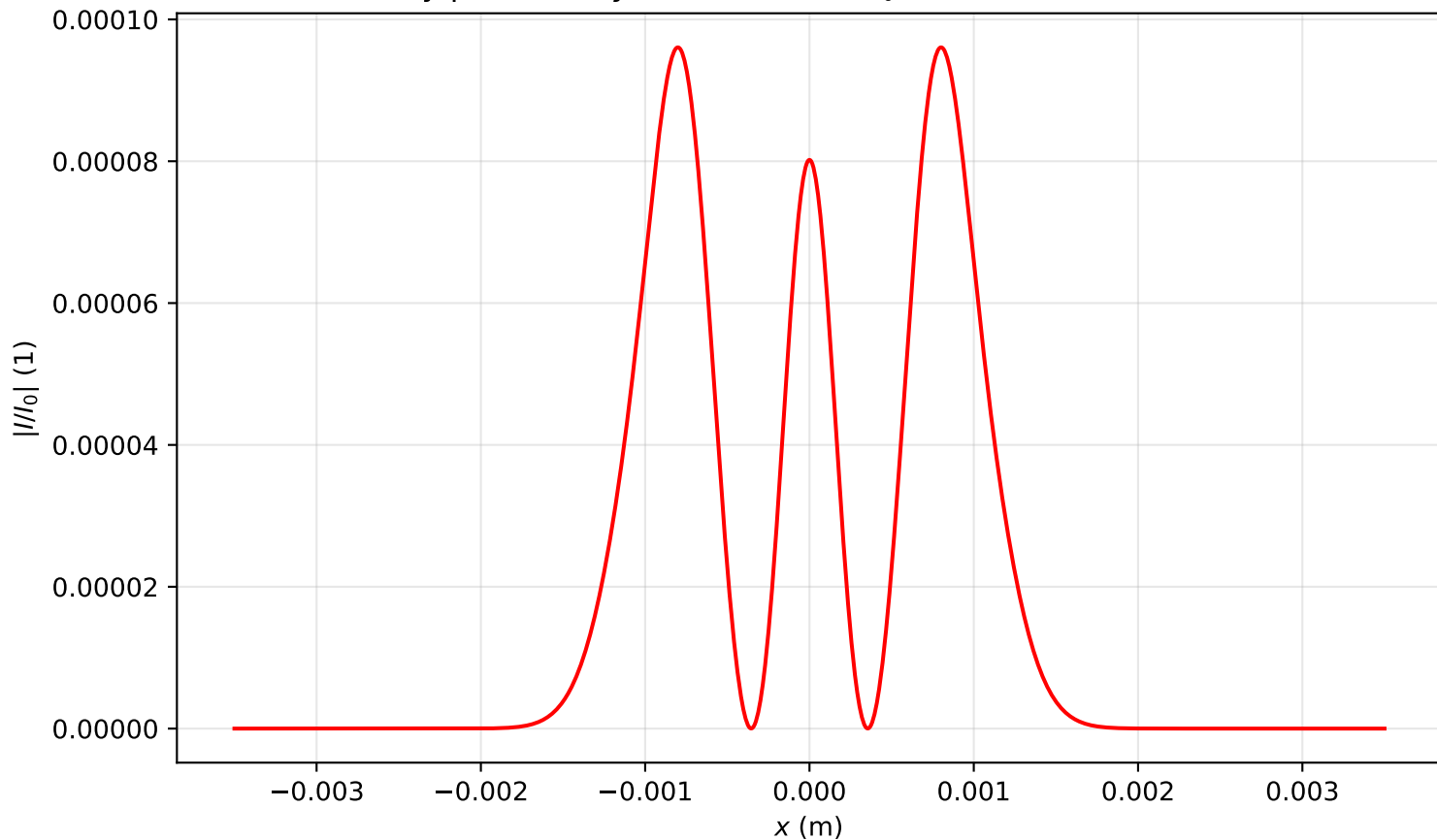
Intensity profile I(x, y = 0, z = 0.398)/I_0 , P_{in}=2.0P_{cr} , artificial time
